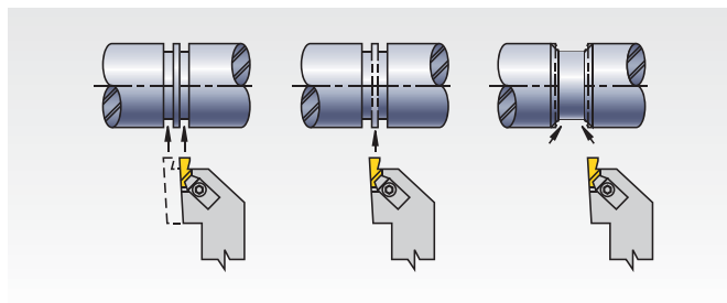
Groove Limits
